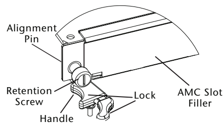
Figure 8: FortiCarrier-5001A left (top) mounting components
