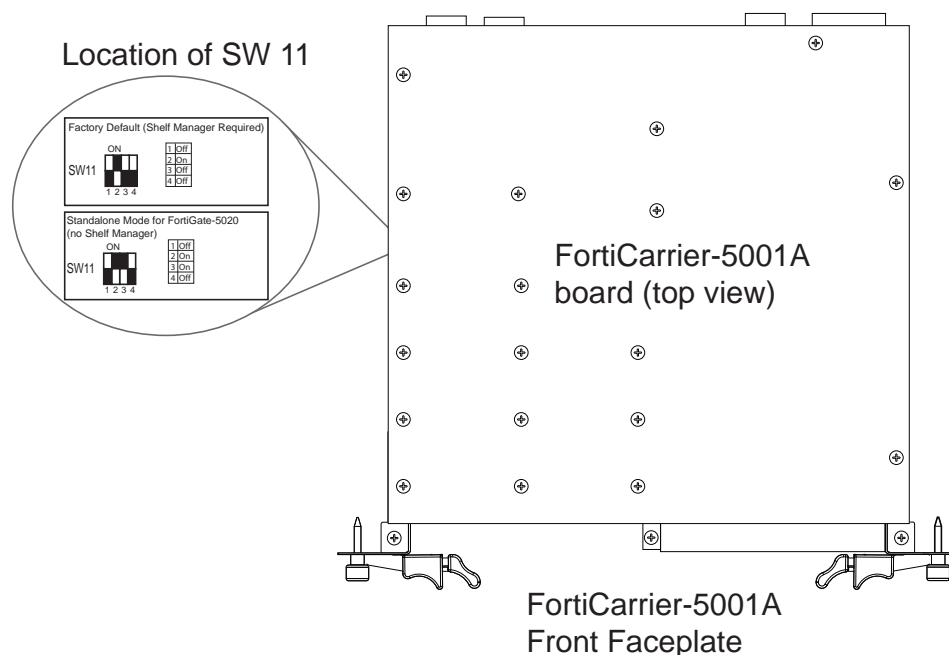
Figure 6: Location of SW11 on the FortiCarrier-5001A board
