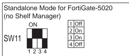
Figure 5: FortiGate-5020 setting for SW11 (standalone mode)
