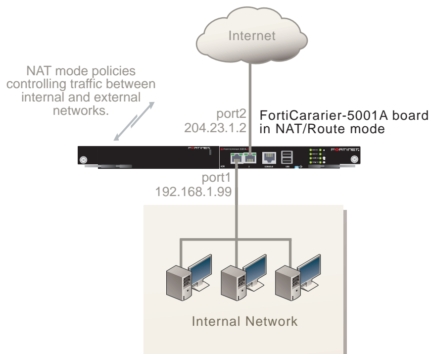
Figure 9: Example FortiCarrier-5001A board operating in NAT/Route mode
