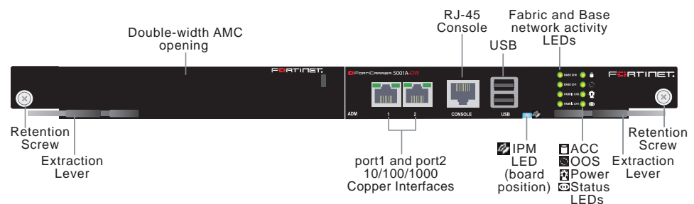
Figure 1: FortiCarrier-5001A-DW front panel
