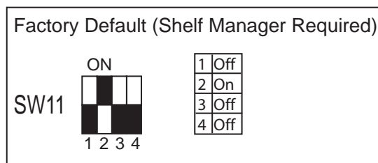
Figure 4: FortiGate-5140 and 5050 setting for SW11 (factory default shelf manager mode)
