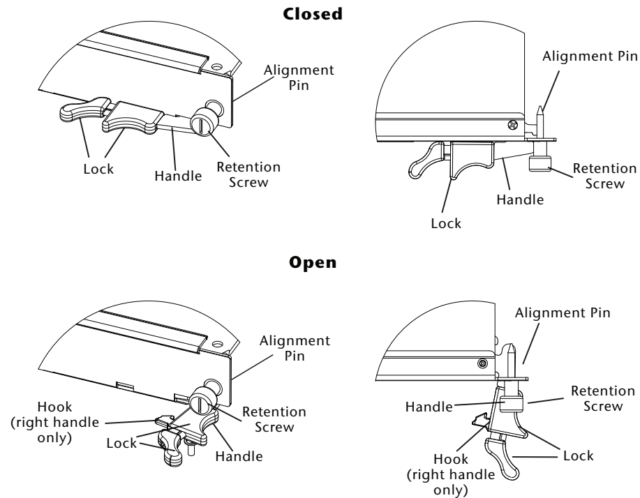
Figure 7: FortiCarrier-5001A right (bottom) mounting components
