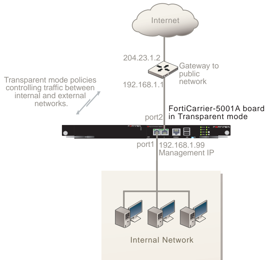
Figure 10: Example FortiCarrier-5001A board operating in Transparent mode
