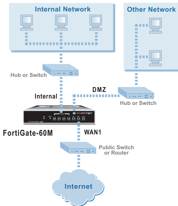
Figure 11: FortiGate-60M Transparent mode connections
