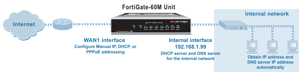
Figure 4: Quick configuration using default settings
