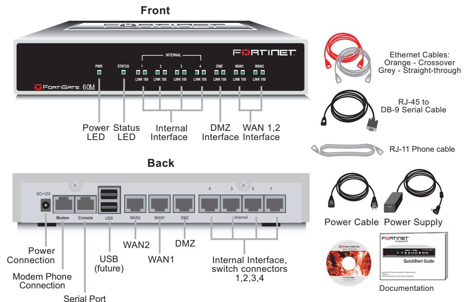
Figure 2: FortiGate-60M package contents
