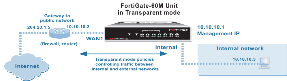
Figure 8: Example Transparent mode network configuration
