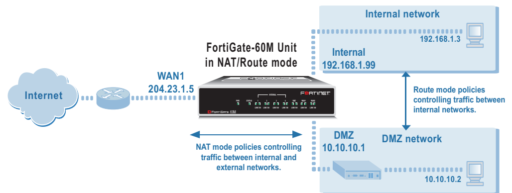
Figure 6: Example NAT/Route mode network configuration
