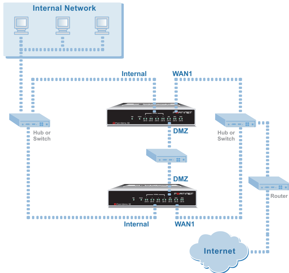
Figure 11: HA network configuration
