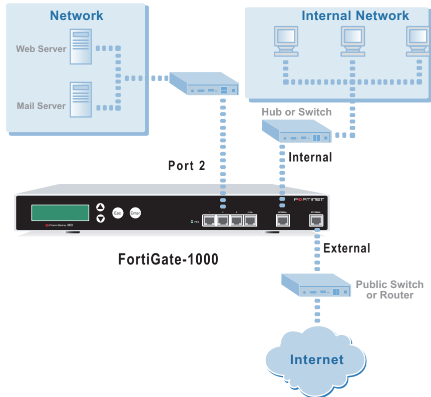
Figure 9: FortiGate-1000 NAT/Route mode connections
