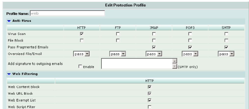
Figure 4: Web protection profile settings
