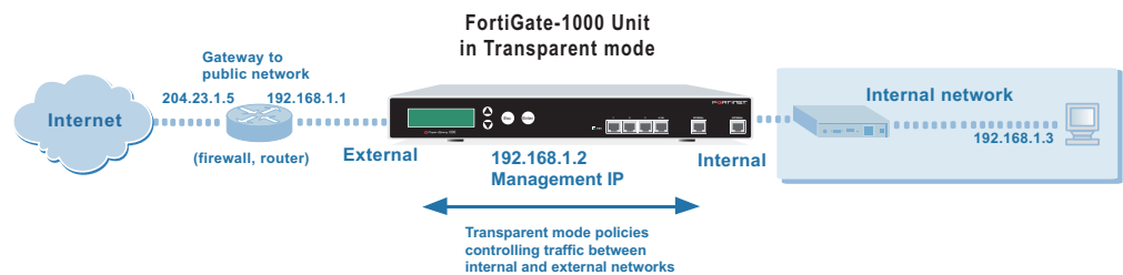
Figure 7: Example Transparent mode network configuration
