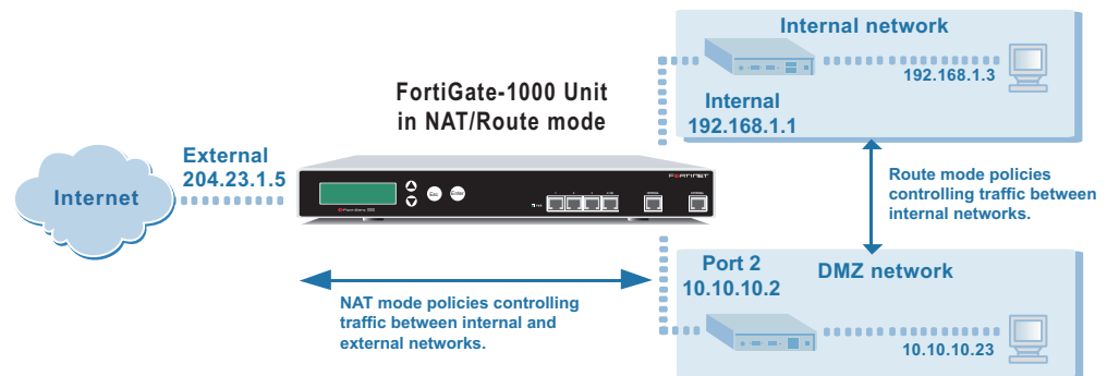
Figure 5: Example NAT/Route mode network configuration
