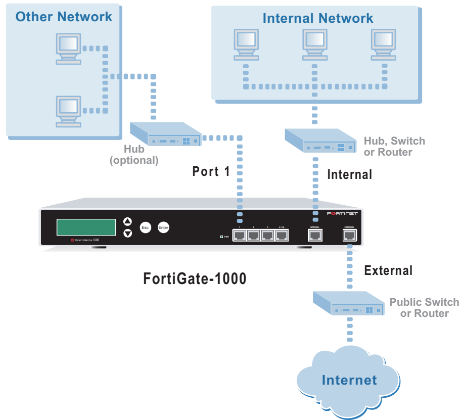
Figure 10: FortiGate-1000 Transparent mode connections
